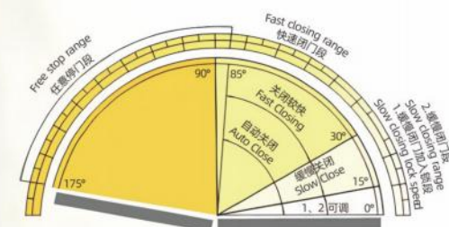
各门类定位功能示意图 Schematic diagram of each door segment positioning function
