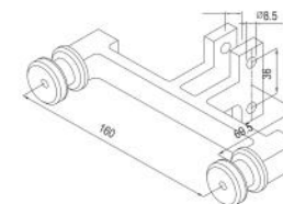
Material:SUS304/SUS316 Stainless Steel Finish:Satin/Polish/PVD
