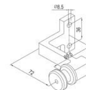
Material:SUS304/SUS316 Stainless Steel Finish:Satin/Polish/PVD
