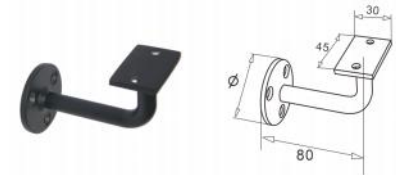
TJ-60 zinc, black powder plated
