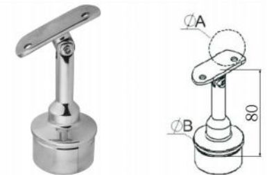
Item NO Ø A Ø B TJ-69-508-508 50.8 50.8
