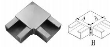
TU-17 Item NO A H TU-17-508254 50.8 25.4 tube slot 15X15mm
