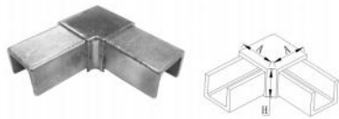
TU-13 Item NO A H TU-13-2521 25 21 tube slot 14X14mm
