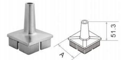
Item NO A TJ-73-381-381 38.1×38.1 TJ-73-508-508 50.8×50.8
