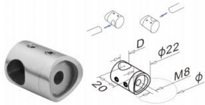
JT-01 closed right/closed left
