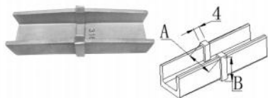
TU-15 Item NO A H TU-15-2521 25 21 tube slot 14X14mm
