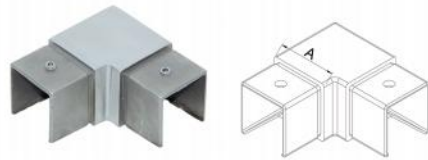
TU-11 Item NO A TU-11-40 40×40 tube slot 24X24mm
