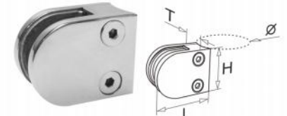
BJ-14 zinc with nickel/chrome plated
