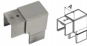
TU-10 Item NO A TU-10-40 40×40 tube slot 24X24mm
