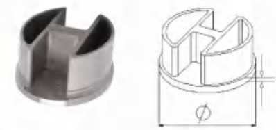
TU-21 Item NO \phi TU-21-508 50.8 double slot 15x15mm
