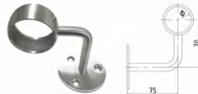
TJ-85 Item NO \phi TJ-85-381 38.1 TJ-85-508 50.8
