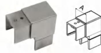
TU-10 Item NO A TU-10-40 40x40 tube slot 24X24mm
