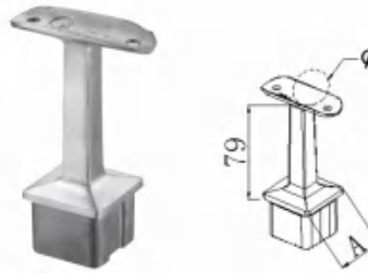
TJ-82 Item NO \phi A TJ-82-424 42.4 40×40
