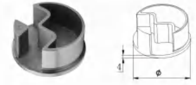
TU-20 Item NO \phi TU-20-508 50.8 90° double slot 15x15mm
