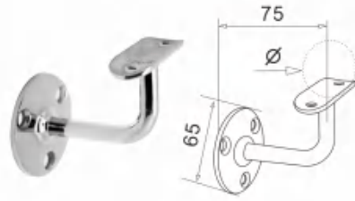
TJ-76 Item NO \phi TJ-76-508 50.8
