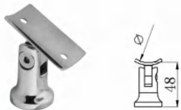
TJ-78 Item NO \phi TJ-78-508 50.8
